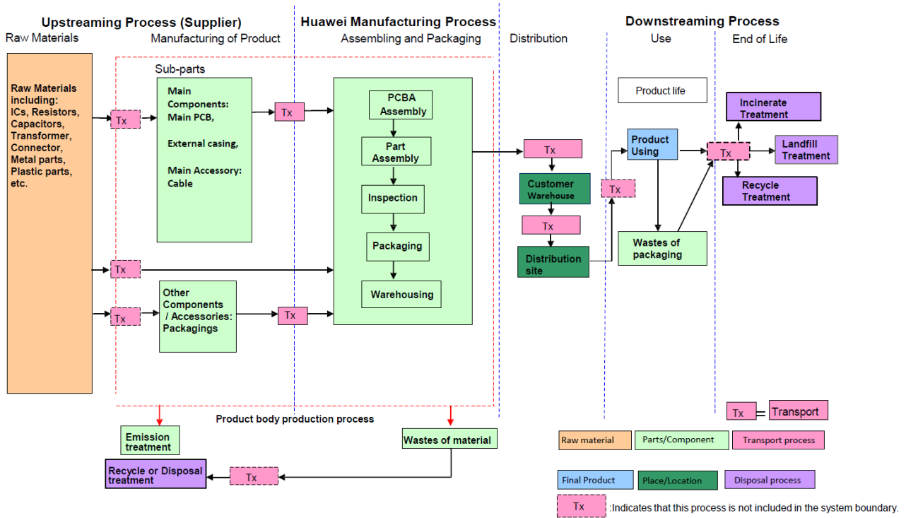
Figure 1 The Life Cycle Process Map of SUN2000-3KTL-M1
