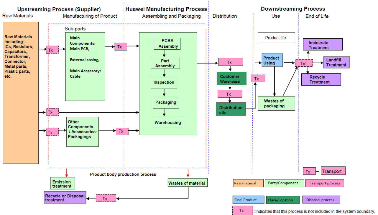
Figure 1 The Life Cycle Process Map of SUN2000-12KTL-M0/SUN2000-12KTL-M2
